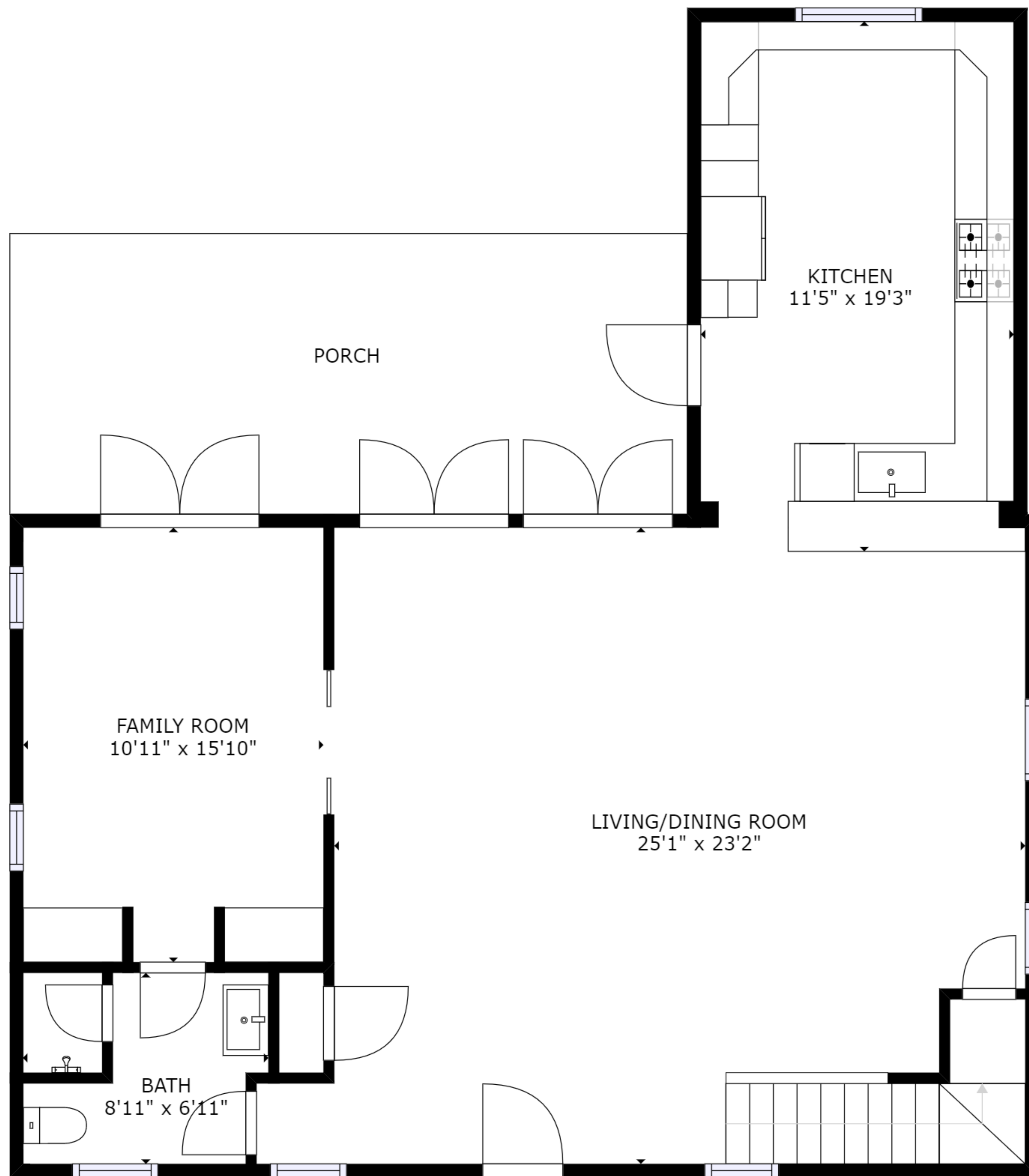
FLOOR 1
